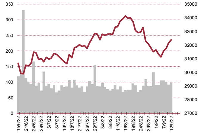
DOW JONES
